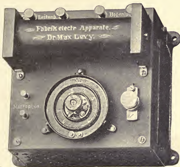
FIG. 27. Regulator for Speaking Arc.
