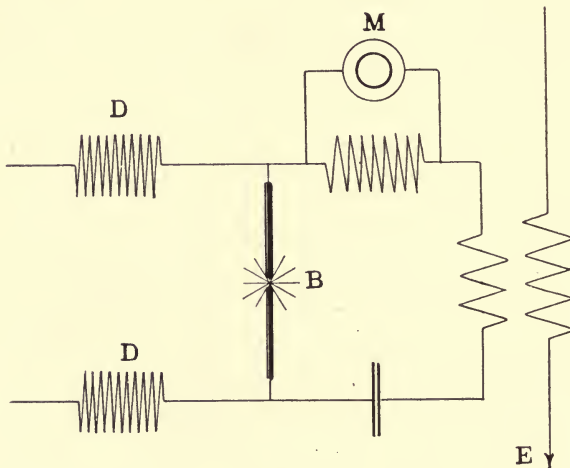
FIG. 115. Campos' Transmitter.
