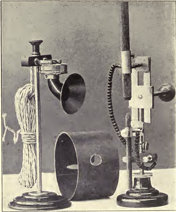
FIG. 26. Speaking Arc Apparatus.
