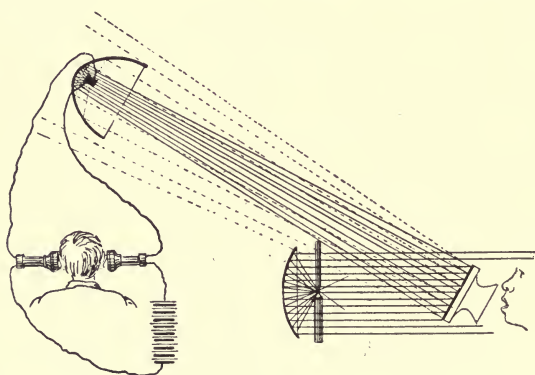
FIG. 5. Arc Lamp as Source of Light.
