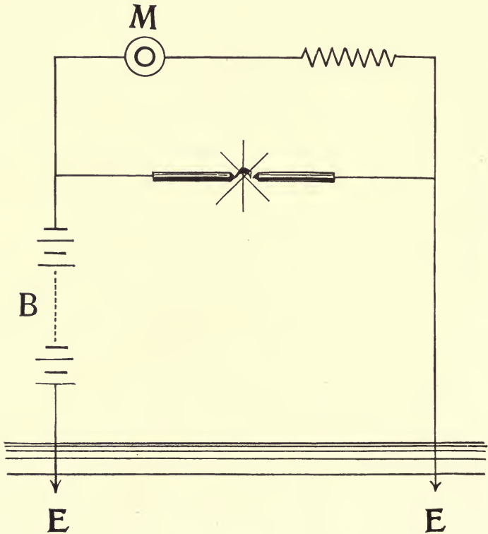
FIG. 66. Arc Transmitter for Closed Circuit System.
