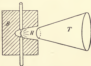
FIG. 28. The Arc as Converter of Sound into Electrical Vibrations.
