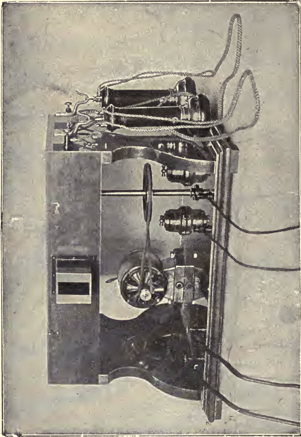
FIG. 37. The Photographophone.
