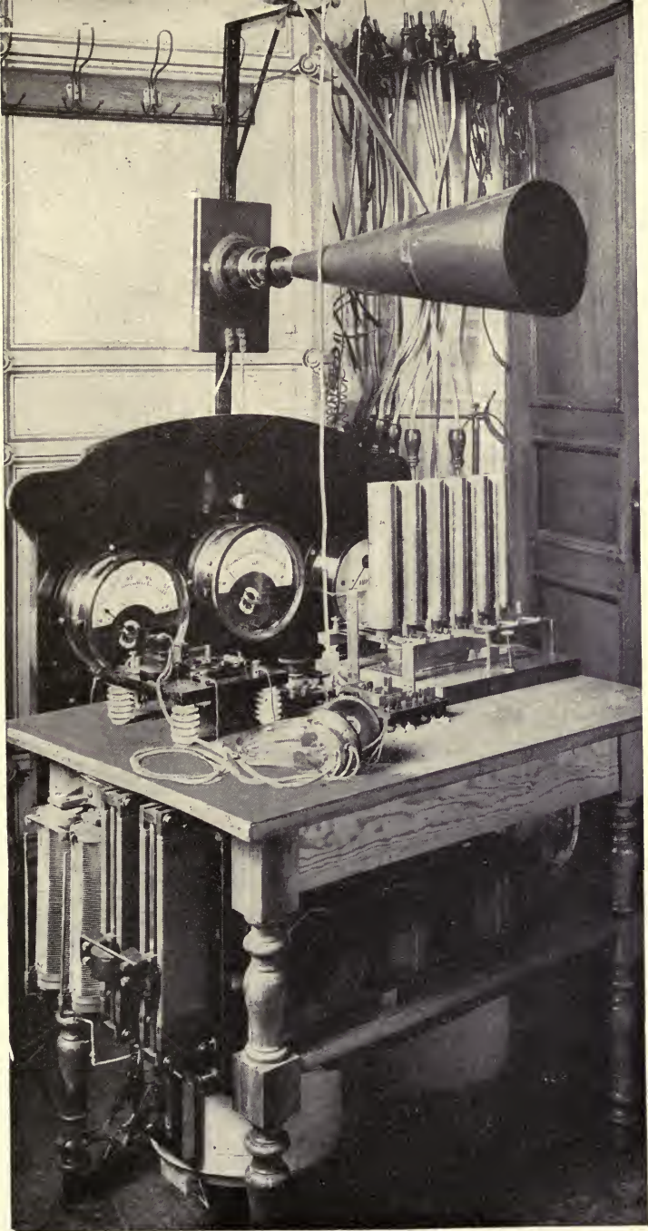
FIG. 127.—Complete Wireless Telephone Apparatus.
