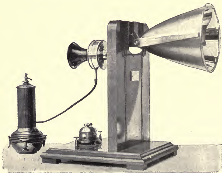
FIG. 17. Experimental Photophones.
