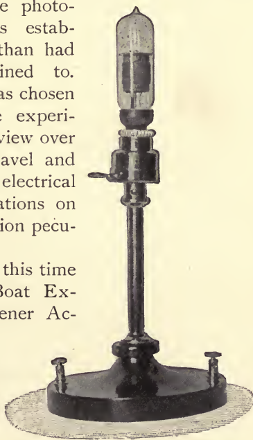
FIG. 40. Cylindrical Selenium Cell Enclosed in Glass Bulb.
