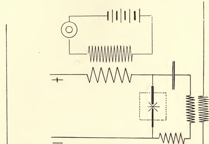
FIG. 125. Ruhmer's Transmitter.
