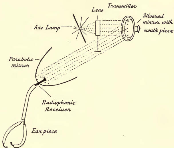
FIG. 8. Thermotelephone.
