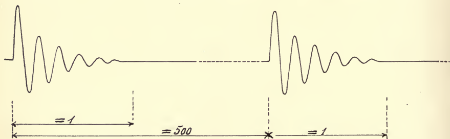
FIG. 83. Damped Wave Trains.
